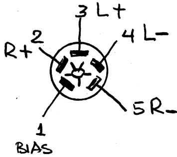
STAX CONNECTOR
